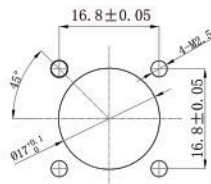
面板开孔尺寸 Panel cutout
